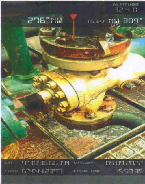
Fig 1: Well 1s Flowline Valve (Incident Valve)
